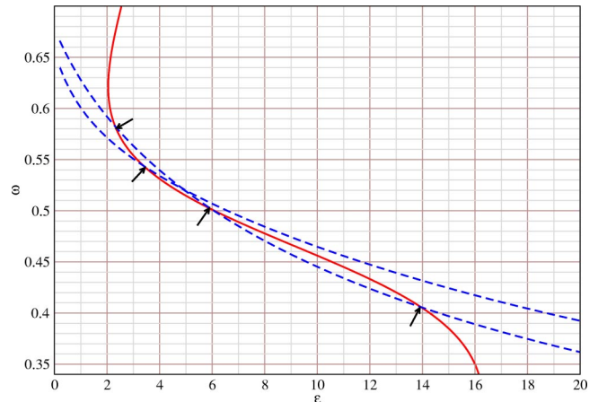
FIG. 14. (Color online) Graphical solution for the calculation of the lowest four frequencies at L point for the system discussed in Fig. 11. The dashed curves represent the frequencies of the lowest two bands as a function of \epsilon as calculated with a frequency-independent method. The continuous curve represents Eq. (8) used to define the “cutting” surface in Fig. 11. The four intersections correspond to the lowest four frequencies at the L point in Fig. 12 or Fig. 13.
