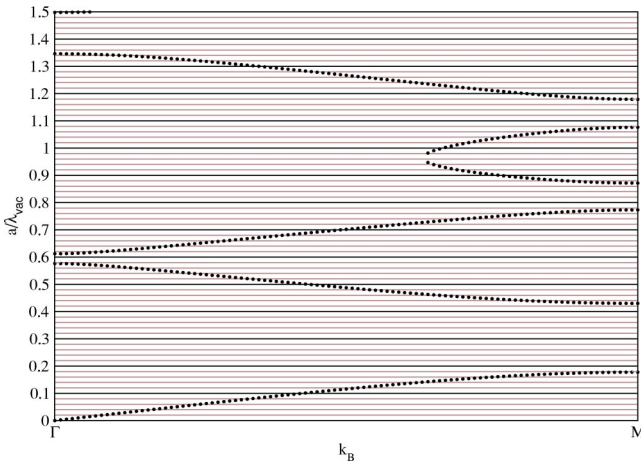
FIG. 18. FDD photonic band structure which exhibits a dispersion bubble at frequencies around \omega|a|/2\pi c = 0.965 . The crystal is characterized by [n_1, |d_1|] = [\text{Re}[\sqrt{\varepsilon(\omega_s)}], 0.2|a|] and [n_2, |d_2|] = [1, 0.8|a|] where \varepsilon(\omega_s) is defined by Eq. (9) with \varepsilon_0 = 12 , \Omega = 2 , \omega_0 = 0.88 , and \gamma = 0.35 .
