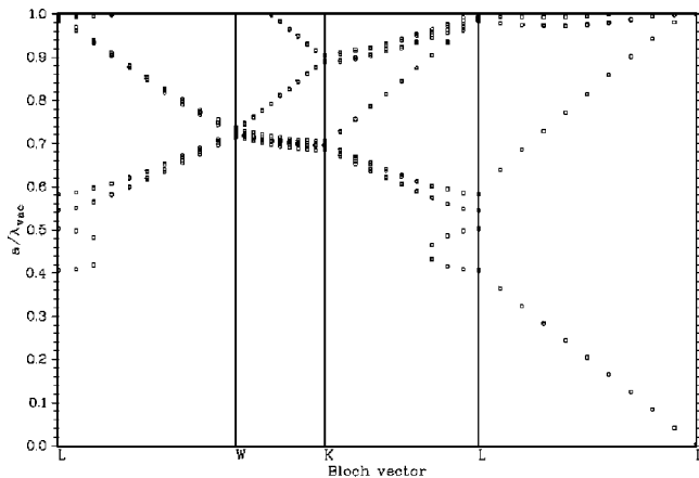
FIG. 12. FDD photonic band structure obtained by projecting the intersections between the “cutting” surface and the band surfaces shown in Fig. 11. A large stop gap (see Fig. 13) opens in the \Gamma - L direction.
