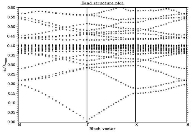
FIG. 10. TM photonic band structure for a polaritonic photonic crystal with solid cylinders of radius 0.472|a| on a square lattice of radius |a| . The cylinders are made from a polar crystal material whose dielectric constant is given by Eq. (5). The parameters used in this case are \varepsilon_0=12.66 , \varepsilon_\infty=10.9 , \omega_T=0.4 , and \gamma=0.01 .
