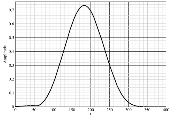
FIG. 22. The input pulse whose intensity profile is shown in Fig. 21 passes through a 1D photonic crystal made from ten unit cells described in the caption of Fig. 18. The pulse is centered at frequency \omega|a|/2\pi c=0.90 . The peak of the input pulse reaches the photonic crystal at t=200 and emerges at x_B at t=184 . This plot shows the absolute value of the amplitude of the output pulse as measured at x_B . In the calculation the imaginary part of Eq. (9) was neglected.
