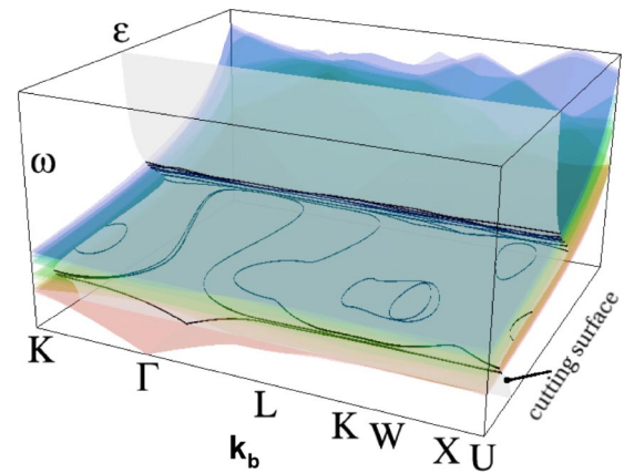
FIG. 16. (Color online) The “cutting” surface is defined by Eq. (8) with the following parameters: \varepsilon_0=12 , \Omega=\sqrt{2} , \omega_0=0.675 , and \gamma_0=0.3 . The band surfaces correspond to an inverted opal of core radius |a|/2\sqrt{2} and \delta_{\text{coating}}=0.08|a| where |a| is the fcc lattice constant. The “islands” created by the intersection between a single band surface and the “cutting” surface give rise to the “closed” bands in the photonic band structure displayed in Fig. 17 above the fourth band.
