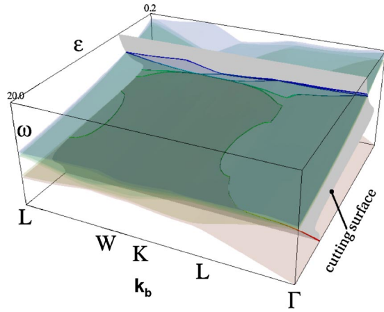
FIG. 11. (Color online) The “cutting” surface is defined by Eq. (8). The band surfaces correspond to a photonic crystal which consists of a fcc close packed arrangement of spheres whose surfaces have been infiltrated with an organic dye. We assume that the dye penetrated only a 10% radial distance inside the spheres. \epsilon runs from 0.2 to 20.
