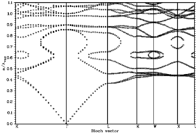
FIG. 17. Photonic band structure obtained by projecting the intersections shown in Fig. 16 on the (\vec{k}_b, \omega) plane.
