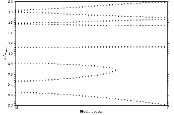
FIG. 27. Band structure of a 1D photonic crystal made from alternating layers characterized by \varepsilon_1(\omega_s) = 10 \sin(4\omega_s) , \varepsilon_2 = 1 , and d_1/|a| = 0.2 . The frequencies are calculated using Eq. (A5) and \omega_s is defined in Eq. (A6). \mathbf{k}_b runs from 0 at \Gamma to \pi/|a| at M .
