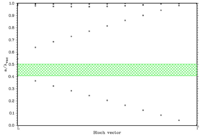
FIG. 13. (Color online) A section of the photonic band structure displayed in Fig. 12 which illustrates the stop gap in the \Gamma - L direction. The relative size of the stop gap ( >20\% ) is much bigger than the one obtained in the absence of the dispersion and is entirely attributed to the placement of the “cutting” surface relative to the band surfaces in Fig. 11. See also Fig. 14.
