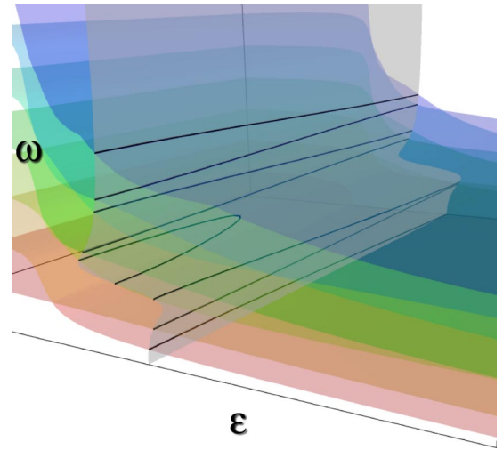
FIG. 19. (Color online) The first six band surfaces and the intersections with the “cutting” surface defined by Eq. (9) with \varepsilon_0 = 12 , \Omega = 2 , \omega_0 = 0.88 , and \gamma = 0.35 . The band surfaces correspond to the 1D photonic crystal described in the caption of Fig. 18.
