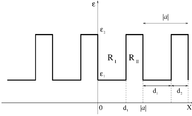
FIG. 26. Spatial profile of the dielectric constant in a 1D photonic crystal. The lattice constant is |a| and the two components are characterized by [dielectric, thickness] of [\varepsilon_1, d_1] and [\varepsilon_2, d_2] , respectively.
