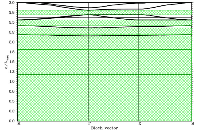
FIG. 7. (Color online) TM FDD photonic band structure for a metallic photonic crystal with the same geometry as the one described in the caption of Fig. 6, except with \omega_p|a|/2\pi c=3 . The flat “pass bands” now appear below the plasma frequency.
