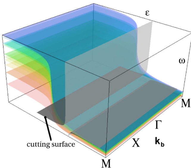
FIG. 9. (Color online) TM photonic band structure of a FDD crystal with a polaritonic resonance described by Eq. (5). The geometry of the crystal is identical with the one used in Fig. 5.
